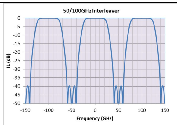
Figure 6 - Designed Spectral Profile of 50/100GHz Interleaver.
