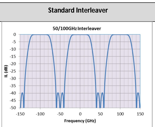
Figure 19 - Standard Interleaver.
