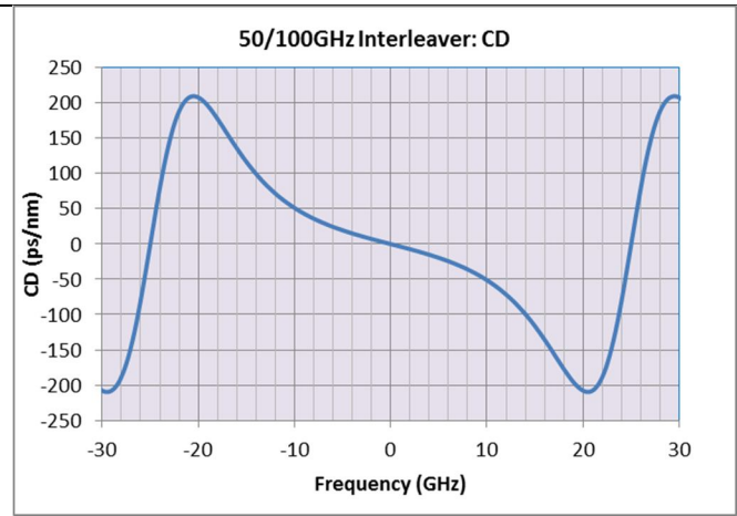
Figure 25 - Zoom-in CD Spectrum of Standard Interleaver.
