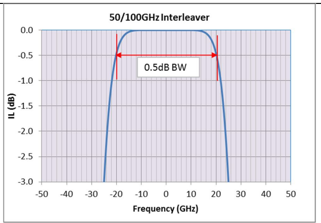
Figure 19 - 0.5dB BW of Standard Interleaver.
