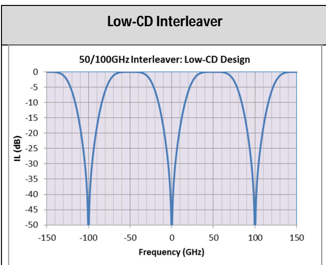
Figure 18 - Low-CD Interleaver.
