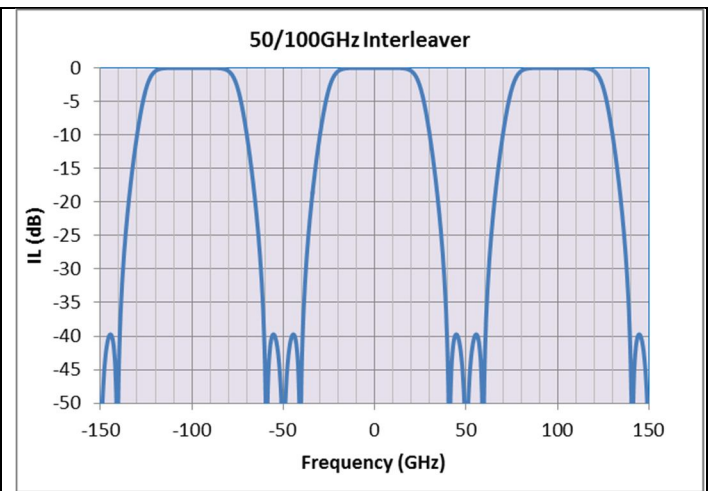
Figure 13 - Standard Interleaver.
