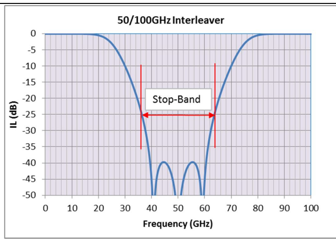
Figure 17 - Stop-Band of Standard Interleaver.
