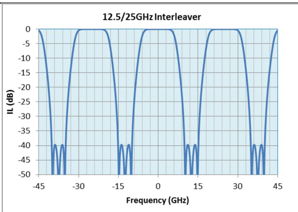
Figure 3 - Designed Spectral Profile of 12.5/25GHz Interleaver.
