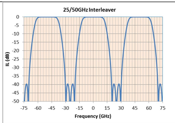
Figure 4 - Designed Spectral Profile of 25/50GHz Interleaver.
