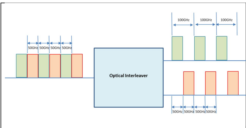
Figure 8 - Symmetric Interleaver Illustration.
