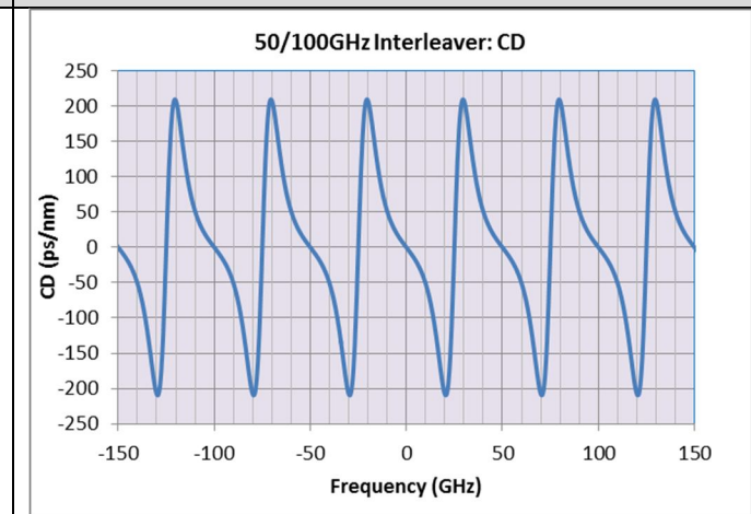
Figure 23 - CD Spectrum of Standard Interleaver.
