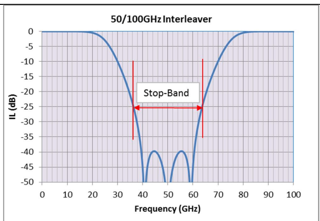
Figure 21 - Stop-Band of Standard Interleaver.
